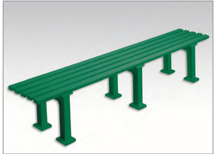
Bench Stuttgart 200 cm long, green 3 plastic legs and 5 multi-chamber plastic slats, without backrest therefore usable from both sides. Practical and comfortable to sit on. Weight approx. 11,5 kg. No. 412213 green
